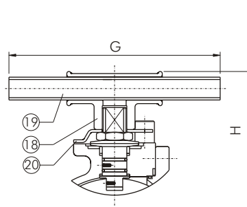
FOR 6" FB CLASS-150
