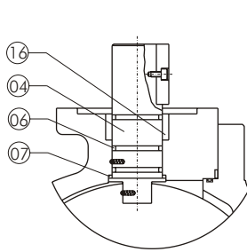
STEM ASSEMBLY DETAILS FOR 6" FB-300# & 8"-150# & 300#
