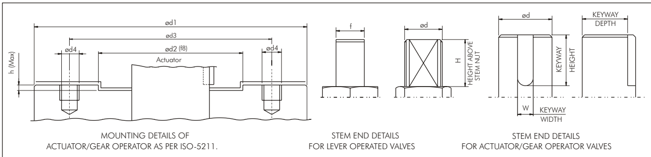
STEM ASSEMBLY DETAILS FOR 6" FB-300# & 8"-150# & 300#
